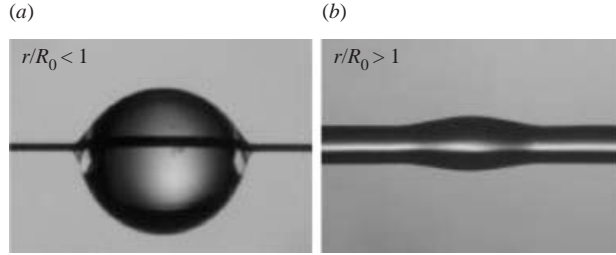
FIGURE 9. Drop of silicone oil (radius R_0 ) on a fibre (radius r ), in the limits (a) r < R_0 and (b) r > R_0 . (a) R_0 = 200 \mu\text{m} and r = 12 \mu\text{m} ; (b) R_0 = 80 \mu\text{m} and r = 100 \mu\text{m} .
