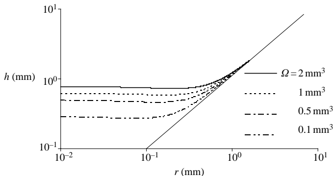
FIGURE 7. Maximum height h of a drop on a fibre, as a function of the fibre radius, for various drop volumes (increasing from bottom to top). For large radii, h tends towards r ( h=r is the oblique line), indicating a flattening of the drop.
