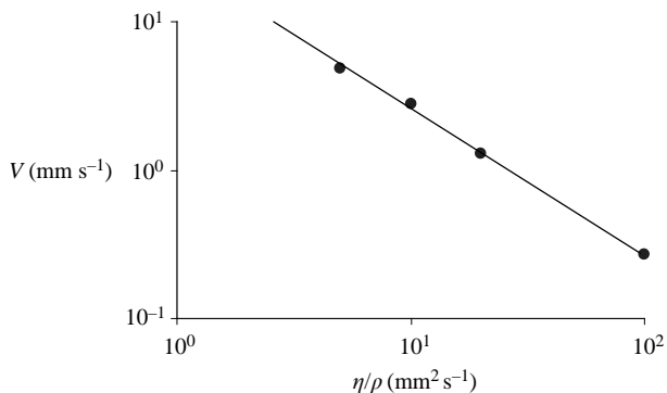
FIGURE 13. Terminal speed of oil drops placed on an inclined fibre as a function of the kinematic viscosity of the oil. The drops are made with silicone oil of various viscosities ( 5 \text{ mPa s} < \eta < 100 \text{ mPa s} ), and all have the same volume \Omega = 0.6 \text{ mm}^3 . The tilt angle is 7^\circ .
